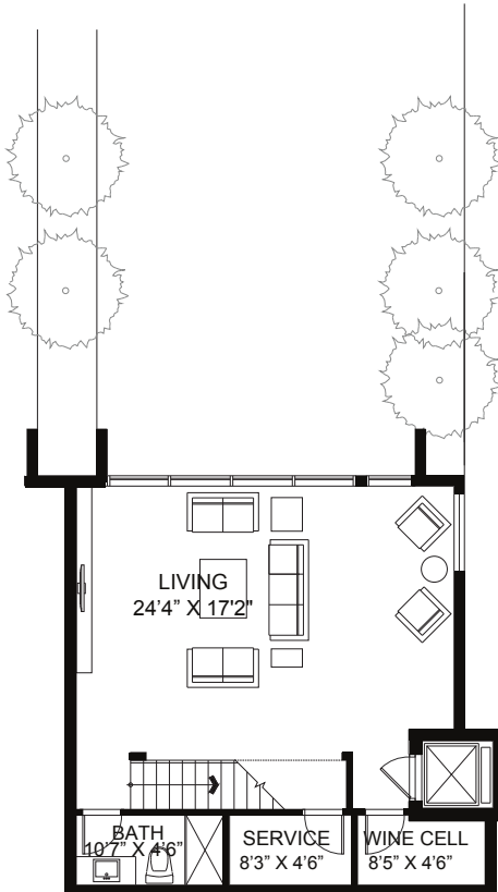
Lower Level Walkout
