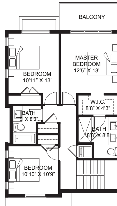
Upper Level
