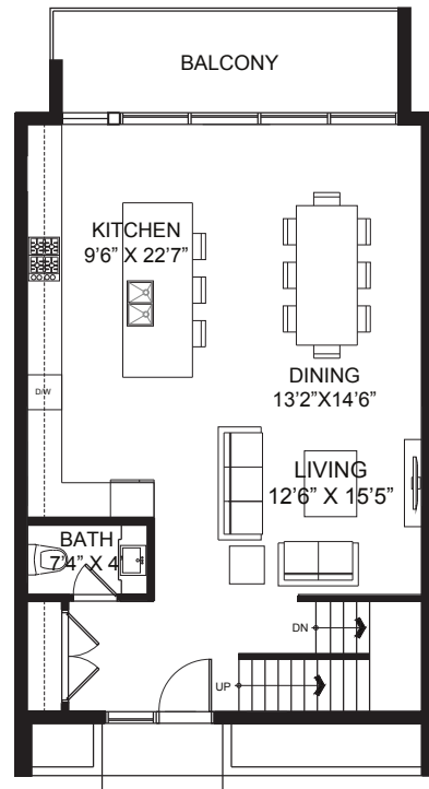
Main Floor
