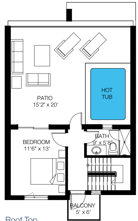
Roof Top
